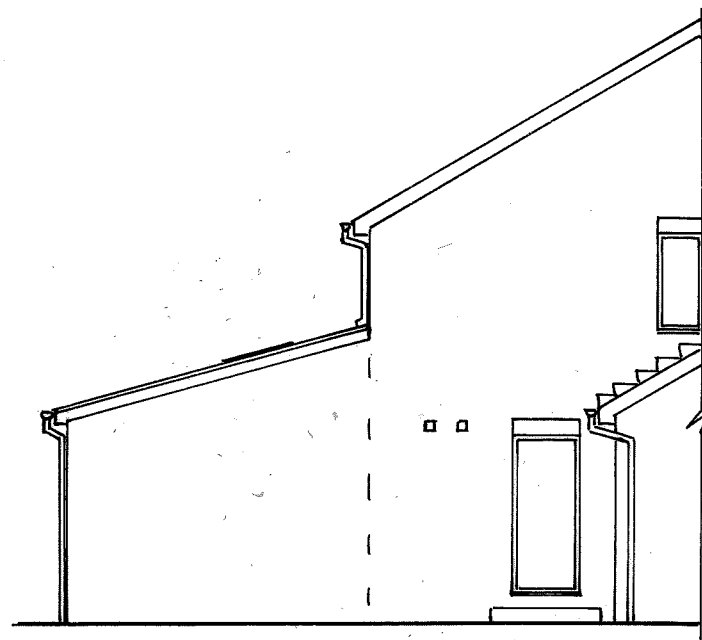
PROPOSED SIDES 1:100
